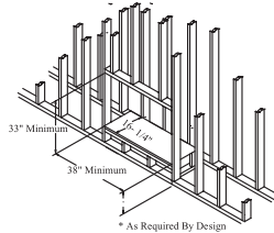
PLATFORM INSTALLATION
