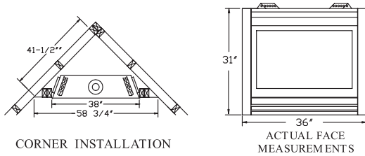
CORNER INSTALLATION
